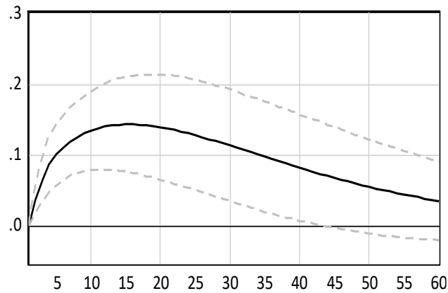
Response of SPREAD to TMS Innovation
