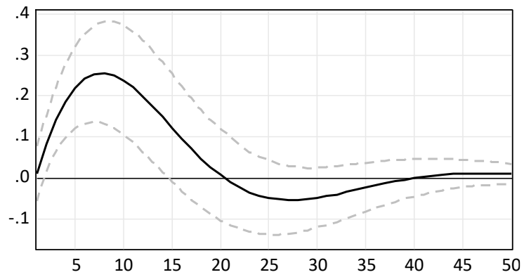
Response of SPREAD to BANKS Innovation
