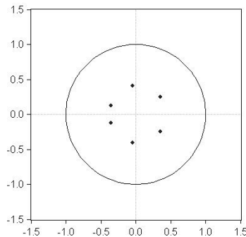
Figure 3 VAR Model Stability Results of CO 2 -GDP-EN for UK (Inverse Roots of AR Characteristic Polynomial)
